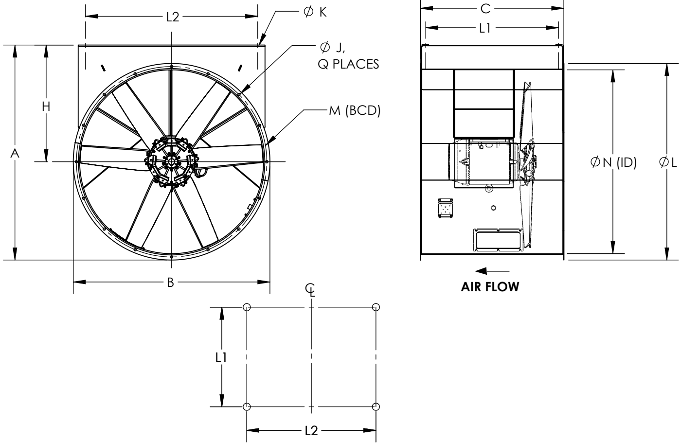
MOUNTING HOLE PATTERN
